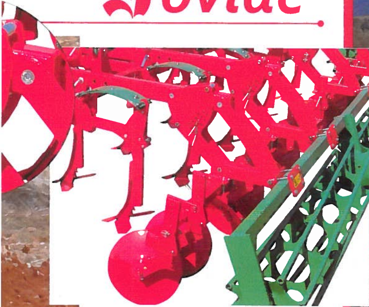
Parallelogram system to adjust discs and rear roller simultaneously
