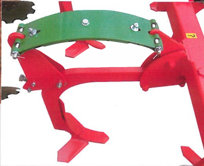
Leafspring auto reset protection. Decreasing trip pressure which protects the key structure of the Versatill. 100% maintenance-free Beams made of wear resistant, high elasticity steel
