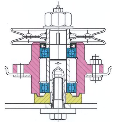
Bearings protected from string, wire, etc.
